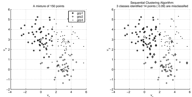
Fig. 5. Misclassification
